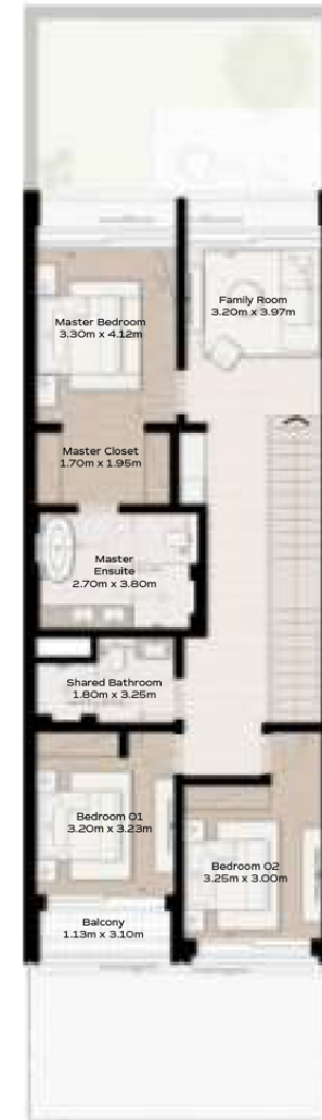
FIRST FLOOR
